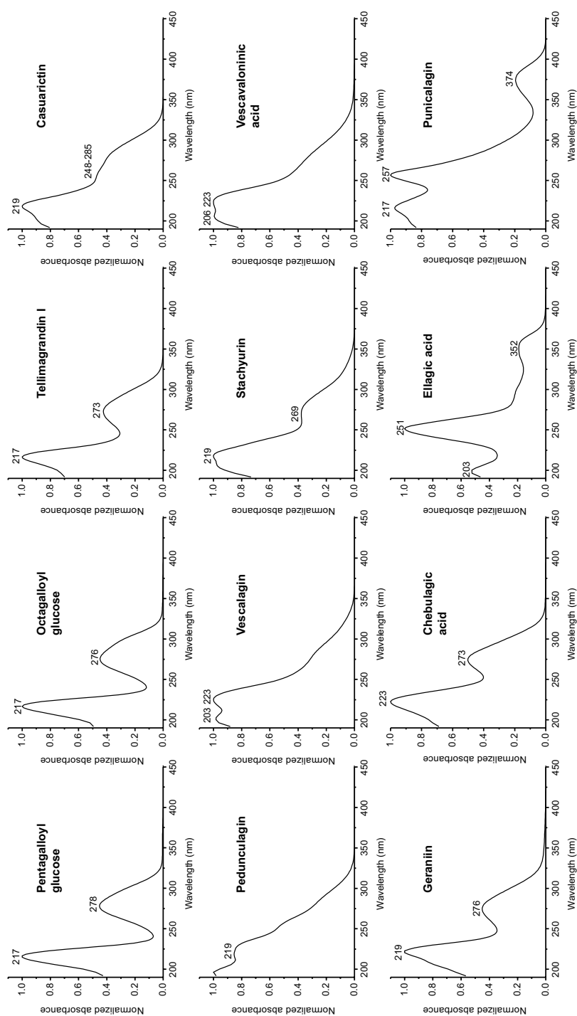
Figure 10. UV spectra of representative compounds belonging to hydrolysable tannin subclasses: galloyl glucoses (pentagalloyl glucose), gallotannins (octagalloyl glucose) and ellagitannins (rest of the spectra).
