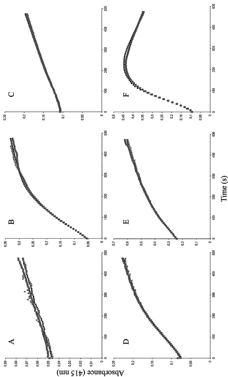
Figure 12. Examples of oxidation curves of selected compounds at 1.5 mM concentration. A = pentagalloyl glucose, B = gallic acid, C = geraniin, D = casuarinin, E = casuarinin and F = vescalonic acid.
