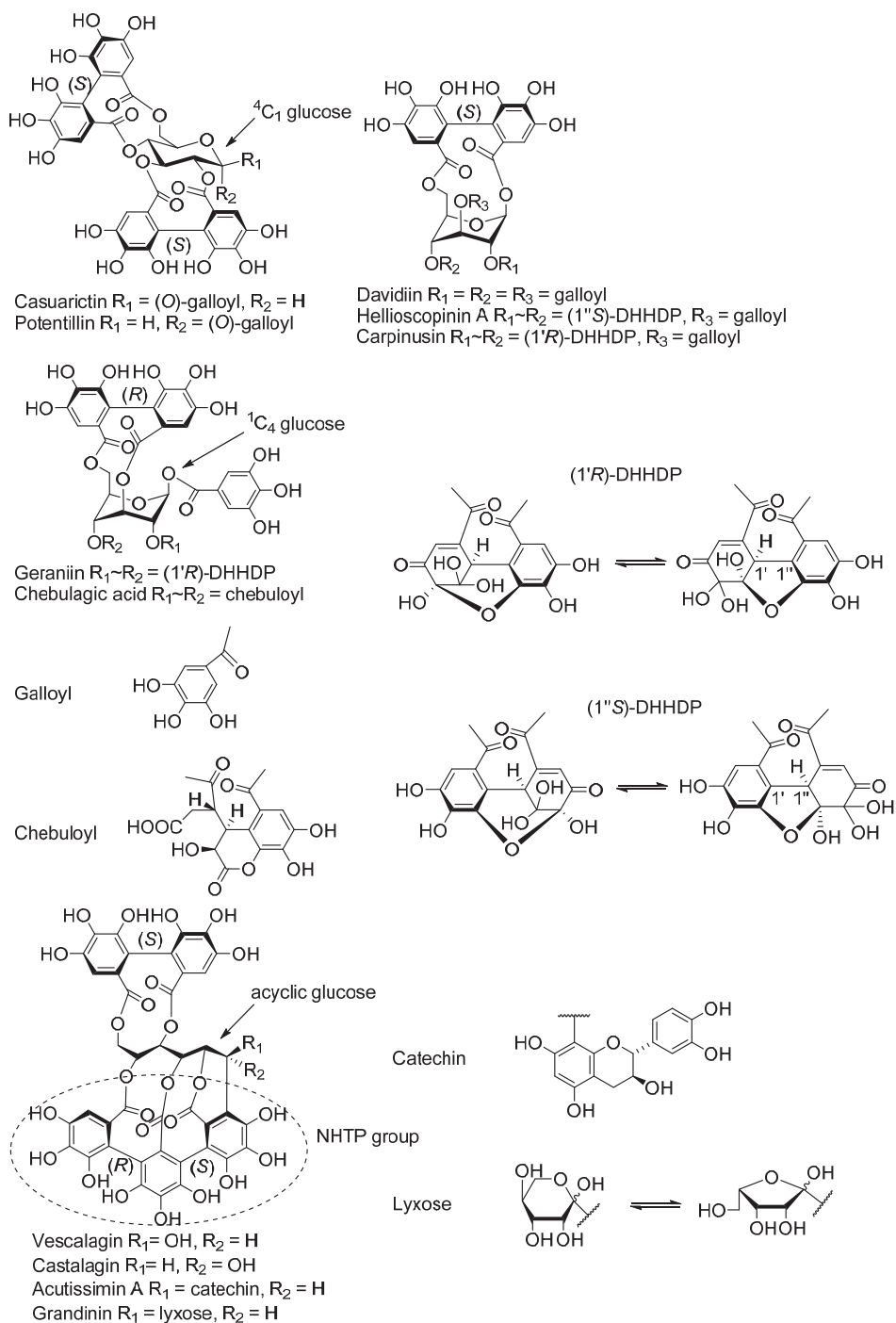
Figure 2. Example structures of monomeric ellagitannins. DHHP = dehydrohexahydroxydiphenyl, NHTP = nonahydroxytriphenyl.
