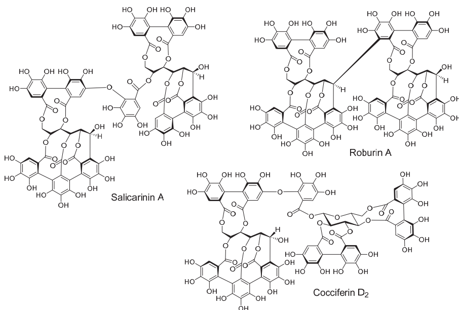
Figure 4. Structural examples of C-glucosidic ellagitannin oligomers.
