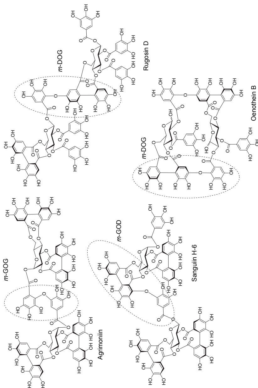
Figure 3. Structural examples of different linking units formed during the oligomerization of ellagitannins. m-GOG = dehydrodialloyl linkage, m-DOG = valoneoyl linkage, m-GOD = sanguisorboyl linkage
