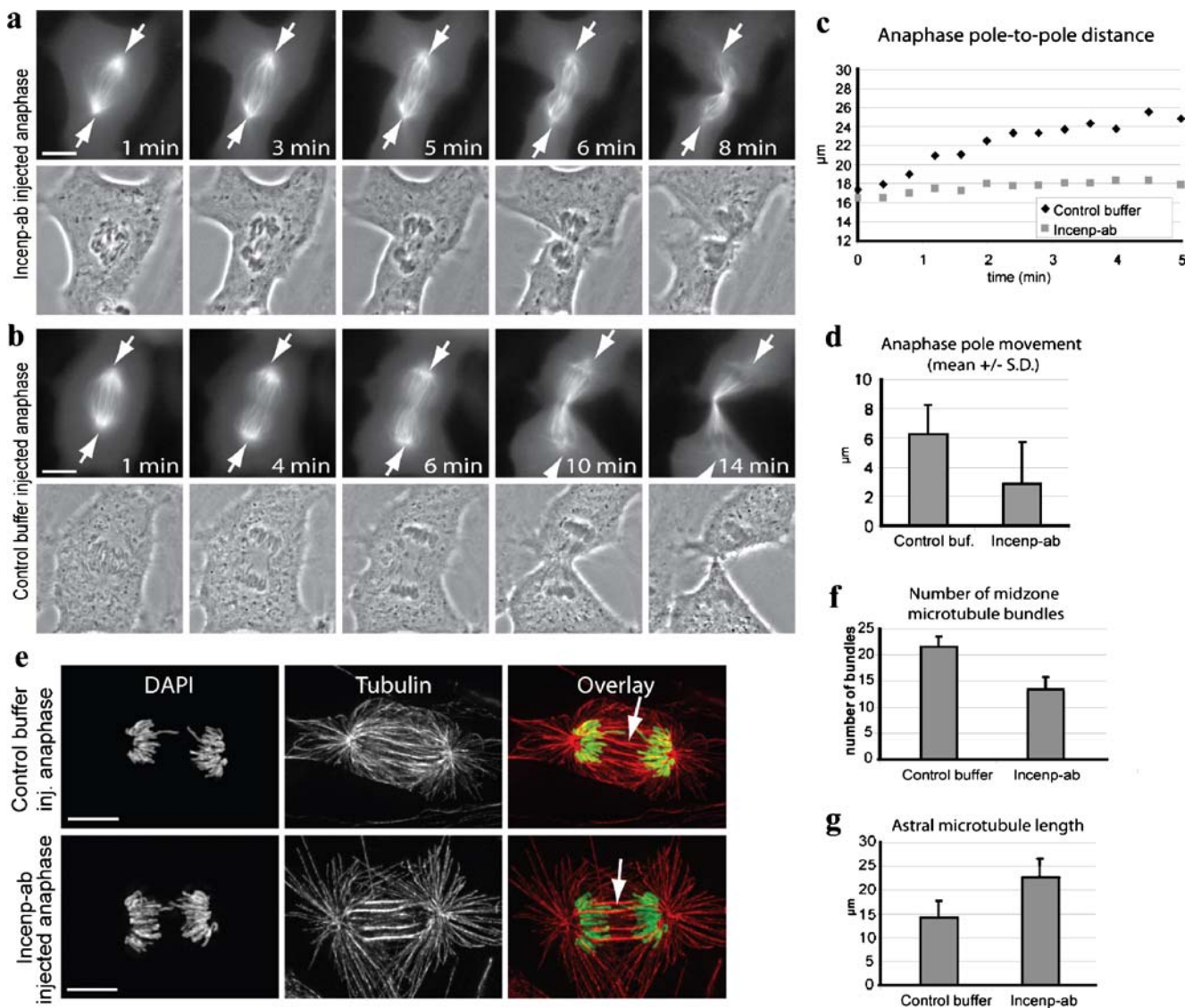
Fig. 5 Incenp ab prevents normal spindle elongation and induces abnormal bundling of midzone microtubules. a GFP-tubulin expressing Xeno S3 cell injected with Incenp ab 1 min after the onset of anaphase shows defects in spindle elongation, spindle pole separation, and anaphase sister chromatid movements (arrows mark spindle poles). b Xeno S3 cell injected with buffer 1 min after anaphase onset shows normal sister chromatid separation and cytokinesis. The first image in panel a and b shows the first frame after injection. The numbers correspond to minutes after anaphase onset. c Spindle pole movements of the cells in panels a and b plotted over time. d Quantification of spindle pole separation in live Incenp ab ( n=5 ) and control buffer ( n=5 )
