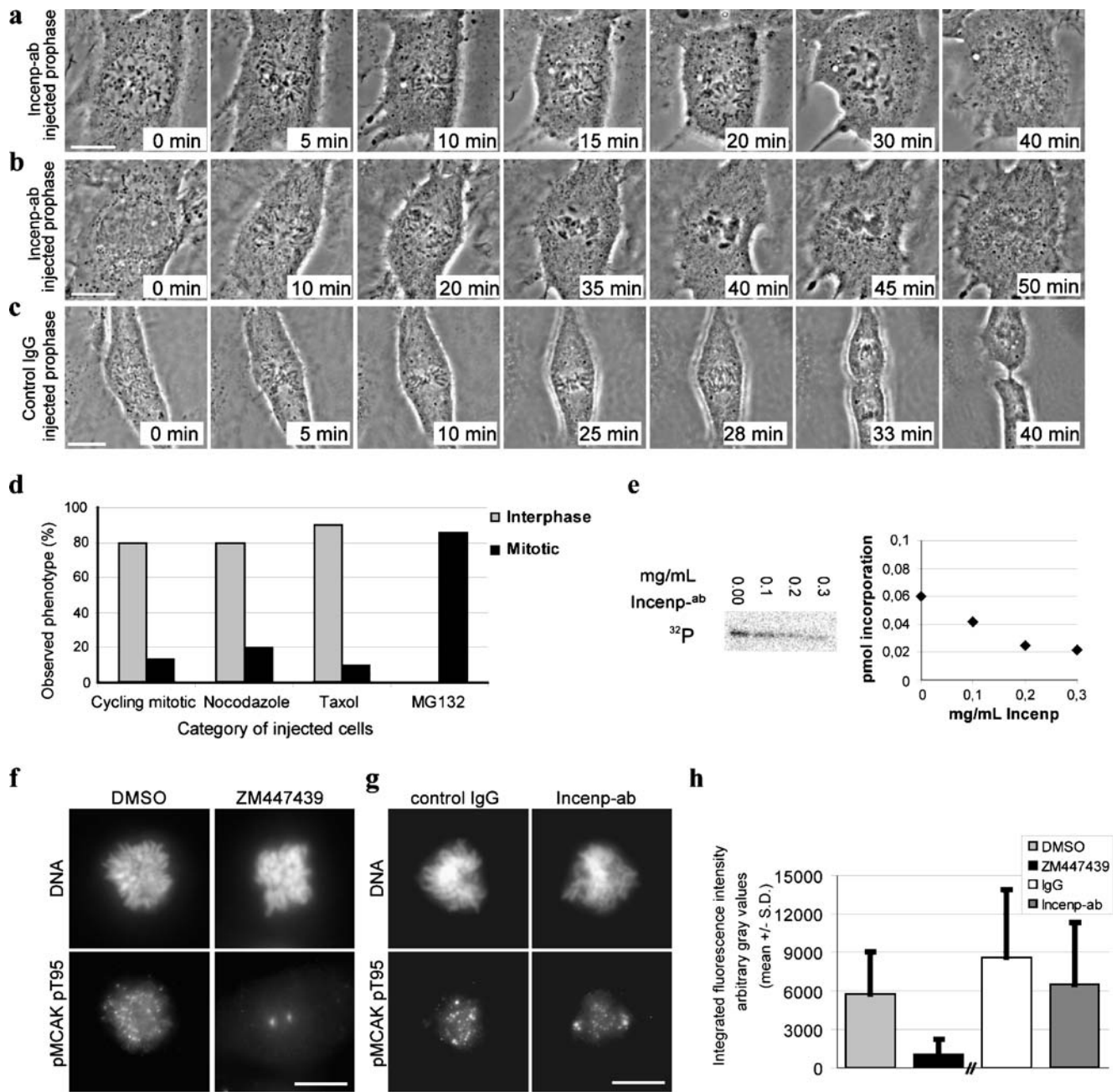
Fig. 1 Injection of Incenp ab into early mitotic cells results in chromosome congression defects and override of SAC. a, b Xeno S3 cells injected with Incenp ab at late prophase. NEB and initial chromosome capture by microtubules appear normal but many chromosomes fail to move to the spindle equator within the time period the chromosomes in control IgG-injected cells ( c ) form a metaphase plate. Chromosomes of the Incenp ab -injected cells undergo premature decondensation and cells exit mitosis without execution of cytokinesis. d Mitotic phenotypes of Xeno S3 cells pretreated with various chemicals prior to introduction of Incenp ab . Cells are categorized as interphase (grey bar) or mitotic (black bar) cells based on their nuclear morphology after the microinjection and subsequent fixation. Most cycling, nocodazole, or taxol-treated cells exit mitosis aberrantly and form polyploid cells with fragmented nuclei indicating
