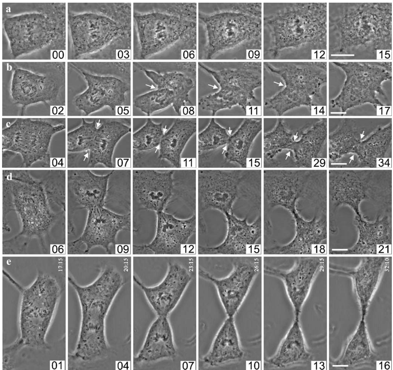
Fig. 4 Interference with Incenp function after anaphase onset disrupts sister chromatid separation and cytokinesis. a Xeno S3 cell injected with Incenp -Δb at the onset of anaphase showing perturbed sister chromatid separation and cytokinesis. b Xeno S3 cell injected with Incenp -Δb 1 min after the onset of anaphase showing incomplete sister chromatid separation and failure of cytokinesis. Cleavage furrow formation (white arrows) is initiated but the furrow soon regresses and the cell exits mitosis forming a polyploid progeny cell. c Xeno S3 cell injected with Incenp -Δb 3 min after the onset of anaphase showing incomplete sister chromatid separation and spindle elongation. Also the cleavage furrow regresses (white arrows) and midbody is not formed. d
