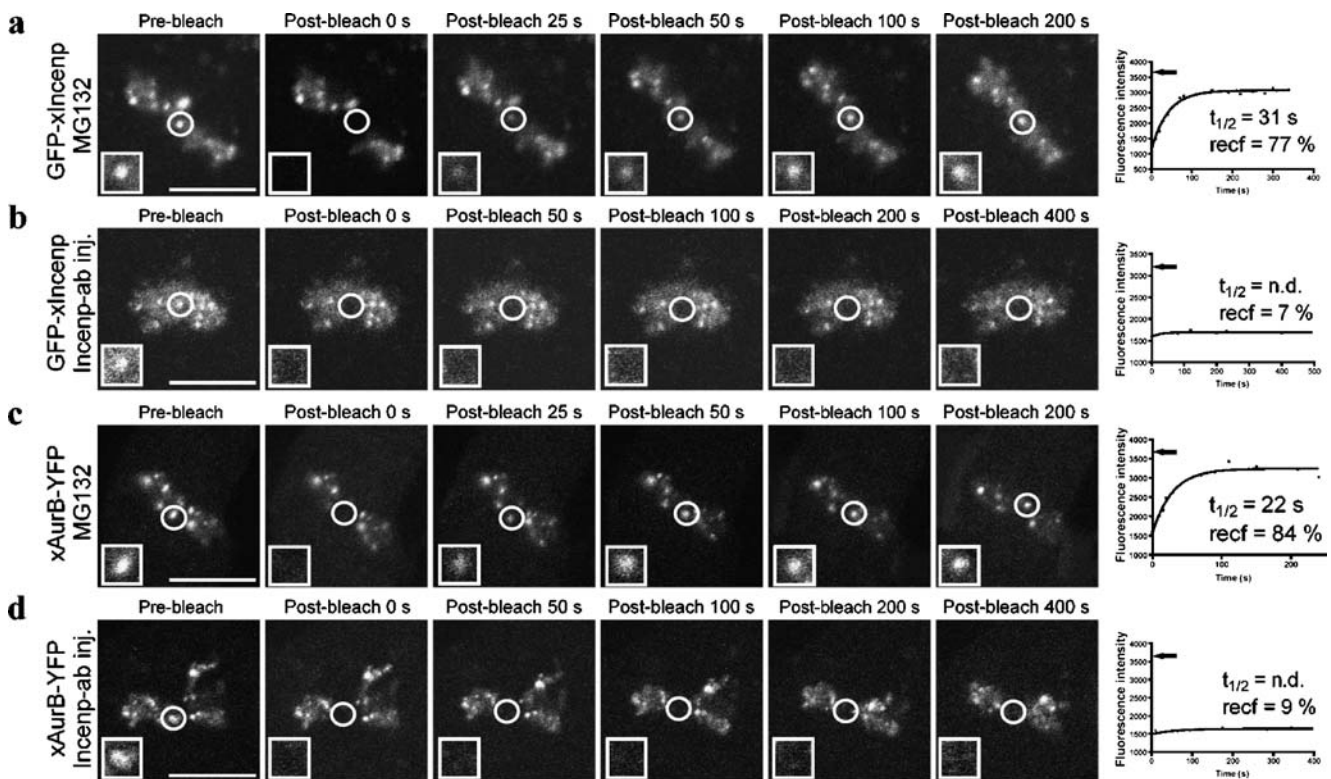
Fig. 3 Incenp ab prevents the dynamic exchange of Incenp and Aurora B at inner centromeres. a, c FRAP analyses of GFP-xIncenp and xAurora B-YFP turnover at the inner centromeres of Xeno S3 cells in the presence of MG132. b, d GFP-xIncenp and xAurora B-YFP turnover after Incenp ab injection in the presence of MG132. Introduction of Incenp ab significantly limits the recovery of both fusion proteins to the photobleached areas. Fluorescent images show fusion protein signal before and at different time points after
