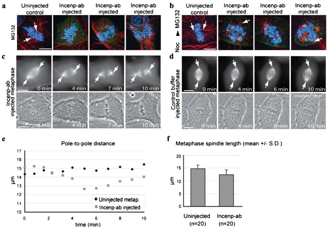
Fig. 2 Incenp ab interferes with the establishment of the mitotic spindle and maintenance of normal spindle length. a, b Images of uninjected control and Incenp ab -injected cells after fixation and staining for microtubules (red), Incenp ab (green), and DNA (blue, DAPI). Prior to fixation the cells were ( a ) treated with MG132 and injected with Incenp ab or ( b ) treated with nocodazole, injected with Incenp ab , and washed out of nocodazole into MG132 containing medium. Incenp ab -injected cells exhibit unorganized spindle morphology characterized by fewer and thinner kinetochore microtubule
