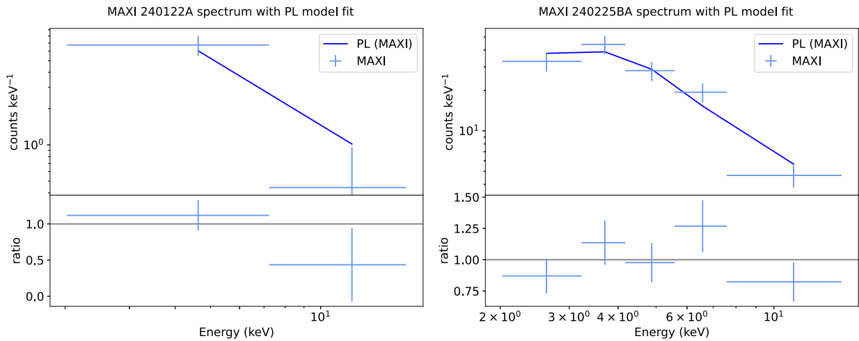
Figure A9. MAXI fitted spectra for GRBs 240122A and 240225B are shown. Models shown are the best-fitting models as described in Table 4.
