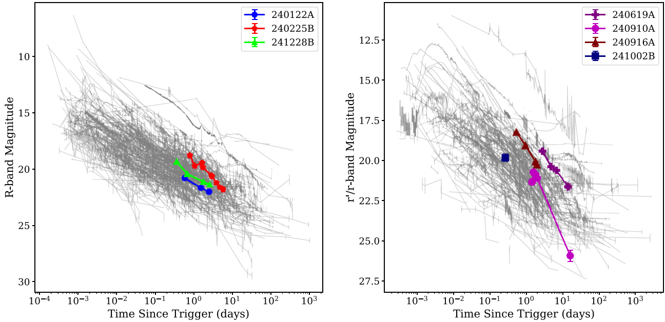
Figure 11. R - and r/r' -band afterglow light curves for the seven GRBs in our sample compared against archival GRB afterglows compiled by M. G. Dainotti et al. (2024), known as the ‘Kann plot’.
