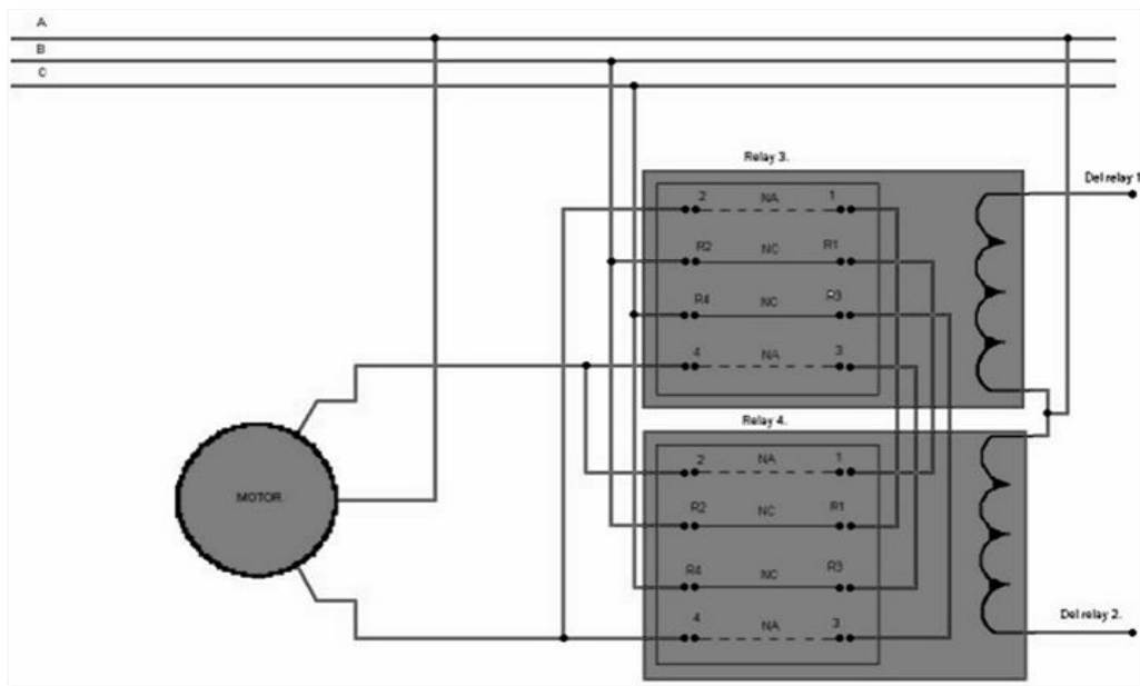
Figure 9. Connection diagram of the relays for control of rotation of the three-phase reversible motor. Source: The authors.
