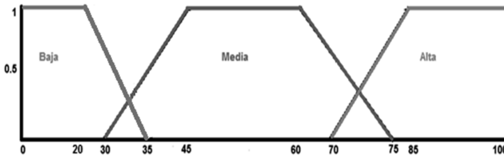
Figure 2. Input membership function (Power). Source: The authors.
