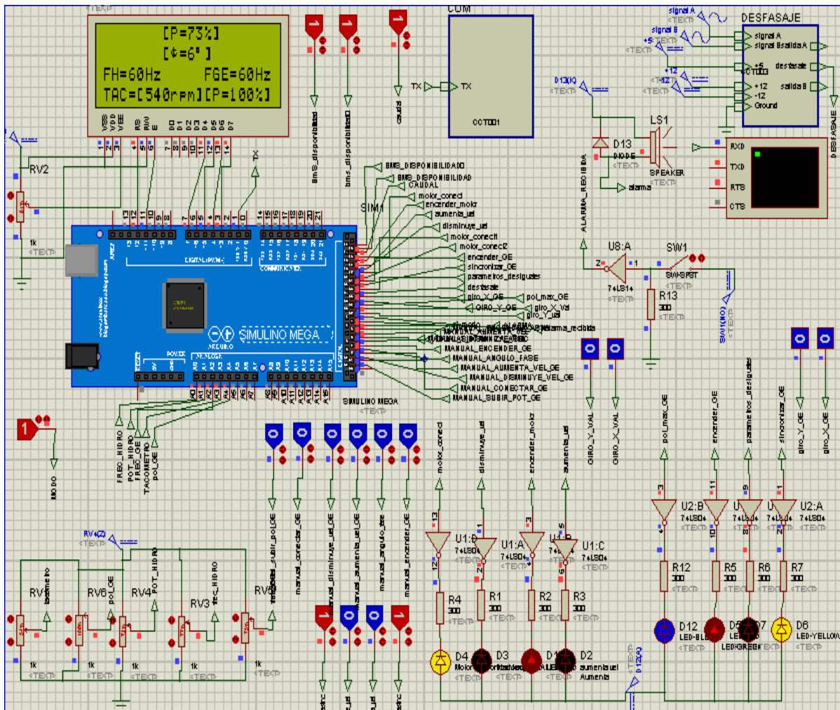
Figure 7. Simulation of the system in Proteus. Source: The authors.
