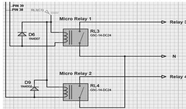
Figure 10. Connection diagram of micro relays 1 and 2. Source: The authors.
