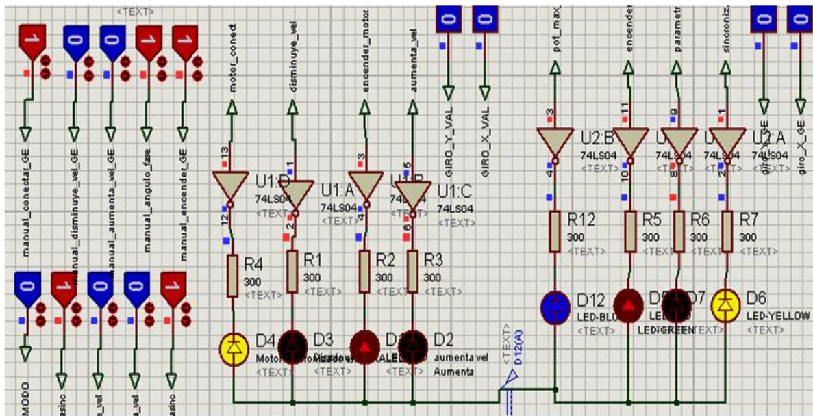
Figure 15. Operation in manual mode of the asynchronous generator and generator set.
