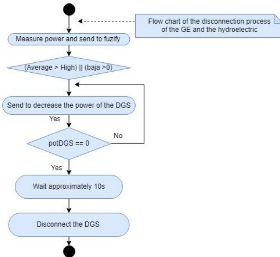
Figure 6. Flow diagram of the disconnection sub-process of the micro hydroelectric plant and the DGS. Source: The authors.
