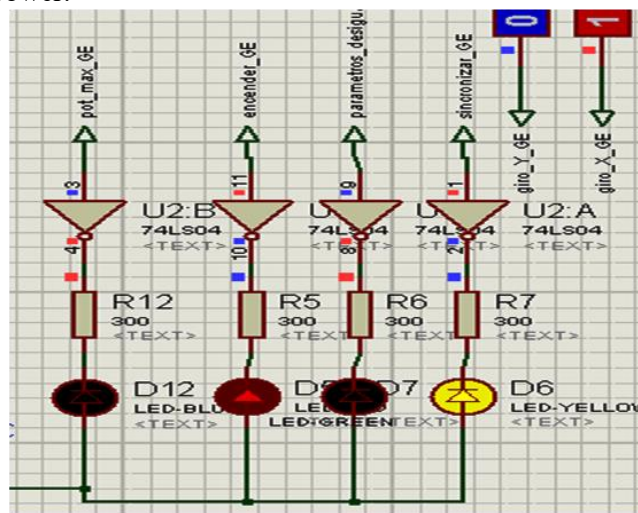
Figure 11. State of the indicators and relays that control the generator set. Source: The authors.
