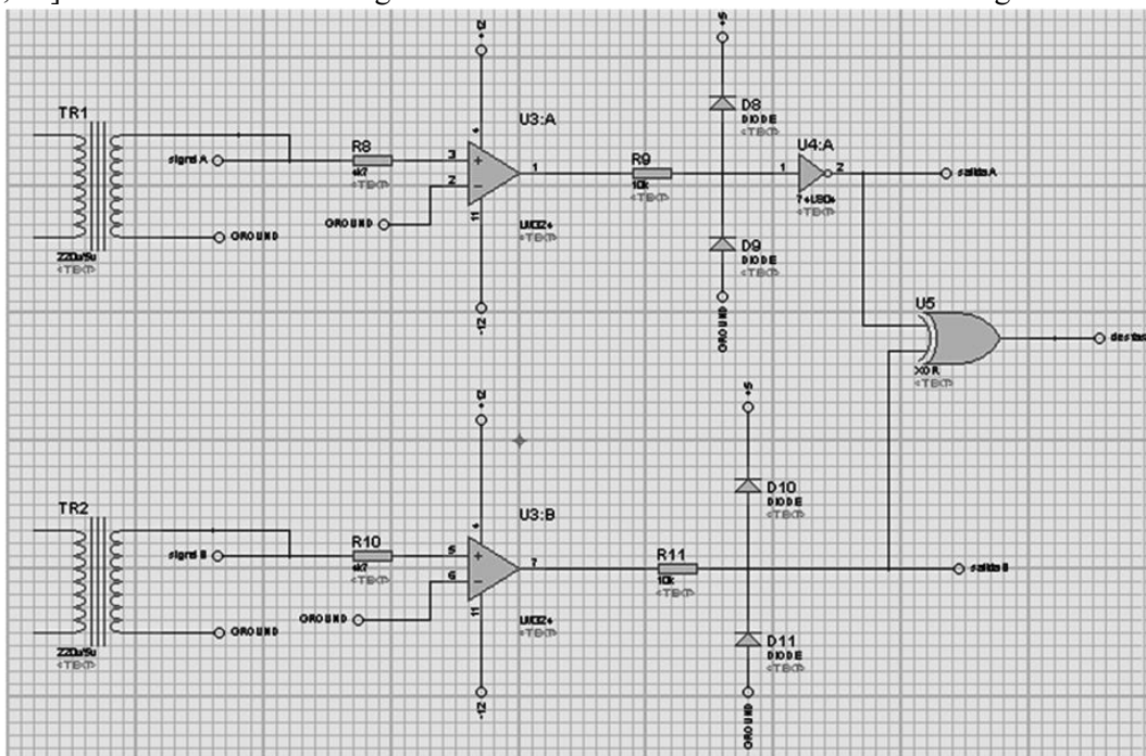
Figure 13. Circuit for phase measurement. Source: The authors.
