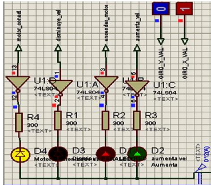
Figure 8. State of the indicators and relays that control the asynchronous motor. Source: The authors.
