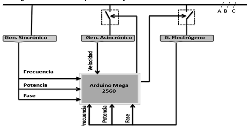
Figure 1. System Blocks Diagram. Source: The authors
