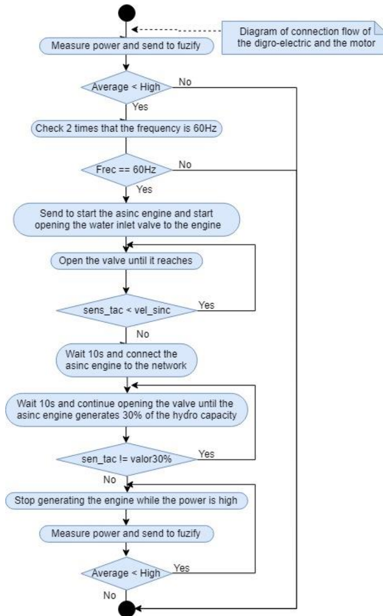
Figure 3. Flow diagram of the connection sub-process of the micro hydroelectric plant and the asynchronous generator. Source: The authors.
