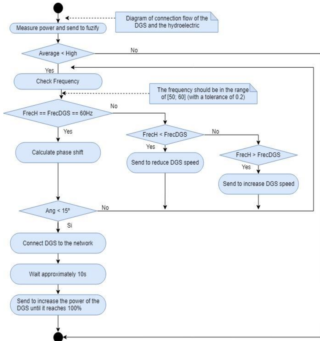
Figure 5. Flow diagram of the connection sub-process of the micro hydroelectric plant and the DGS. Source: The authors.
