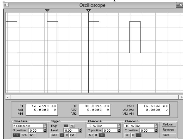
Figure 14. Circuit output signal for phase measurement. Source: The authors.
