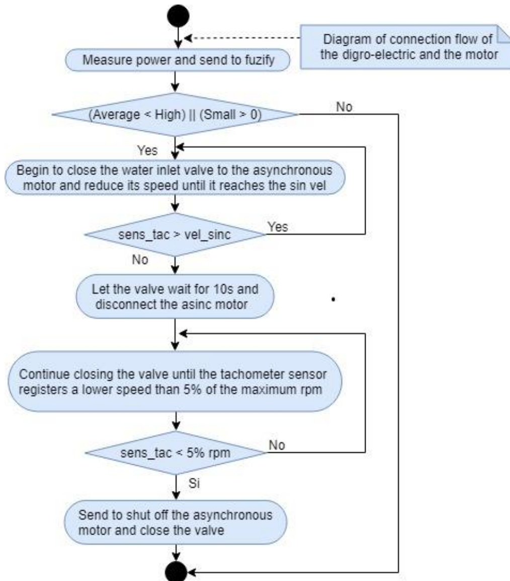
Figure 4. Flow diagram of the disconnection sub-process of the micro hydroelectric plant and the asynchronous generator. Source: The authors.
