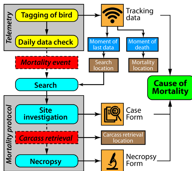
FIGURE 1 | Schematic representation of the process to determine the cause of mortality of GPS-tagged red kites ( Milvus milvus ) as part of the LIFE EUOKITE assessment protocol (LEAP): Data collection starts with tagging the bird, followed by daily data checks for signs of mortality. If a mortality event occurs, tracking data provides an accurate moment and location of death. This triggers searching for a fresh carcass quickly, with the search location determined from the last known tracking data point. A fresh carcass provides a better chance of carrying out a successful necropsy evaluation. The mortality cause is determined based on three sources: (1) tracking data, (2) observations during the site investigation (documented in the Case Form) and (3) necropsy results (documented in the Necropsy Form). The coloring reflects the following categories: Yellow—GPS tracking; red—event related to the focal carcass; cyan—performed actions during the investigation; orange—information sources for the assessment; blue—point in time; brown—location; green—result of assessment.
