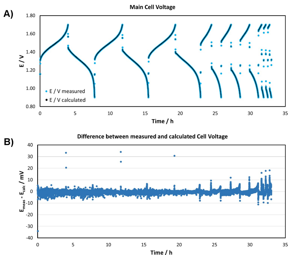
Figure 7. A) Comparison of the recorded main cell voltage values against the calculated values during the cycling experiments of the VFB1. B) Difference between the measured ( E_{meas} ) and calculated ( E_{calc} ) cell voltage.
