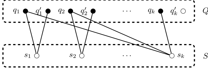
Figure 1: The construction of graph G_k in the proof of Proposition 6, with an optimal LTD-set (black vertices).
