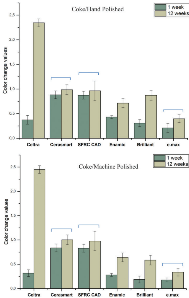
Figure 4. The mean colour change ( \Delta E ) values of the CAD/CAM materials measured after 1 and 12 weeks of immersion in coke, considering both hand and machine polishing techniques. Polishing technique showed no significant effect ( p > 0.05 ) and groups joined by a line are not significantly difference.
