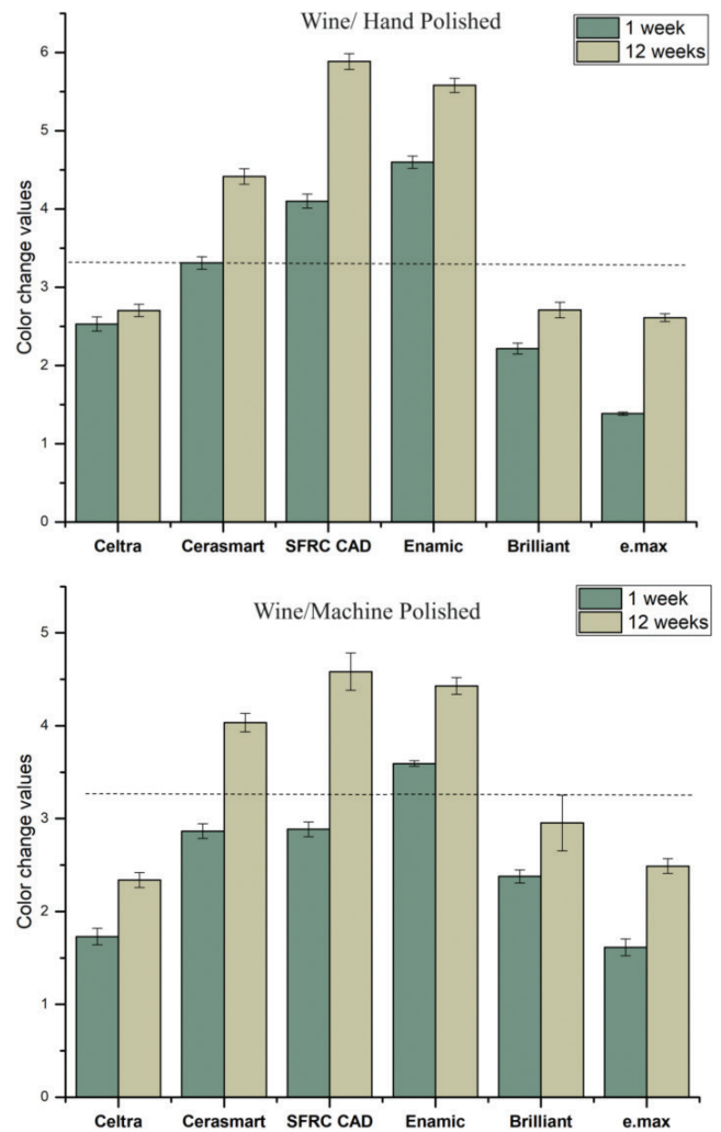
Figure 3. The mean colour change ( \Delta E ) values of the CAD/CAM materials measured after 1 and 12 weeks of immersion in red wine, considering both hand and machine polishing techniques. Values that are higher than the dotted line suggest clinical unacceptability, with a threshold of \Delta E \geq 3.3 .
