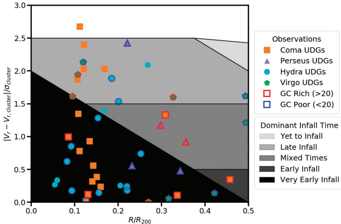
Figure 2. Infall diagnostic diagram for only UDGs in the Hydra I, Coma, Virgo, and Perseus clusters. Regions of the diagram are shaded according to their infall times from the cosmological simulations of Rhee et al. (2017). As per the legend, UDGs in different clusters are denoted by different symbols. Symbols are outlined in red (if GC-rich) or blue (if GC-poor), and without an outline if the GC properties are unknown. See main text for discussion of selection effects in the UDG samples. GC-rich UDGs are not predominately found in the very early infall region, indeed the data suggest that very early infall UDGs tend to be GC-poor.
