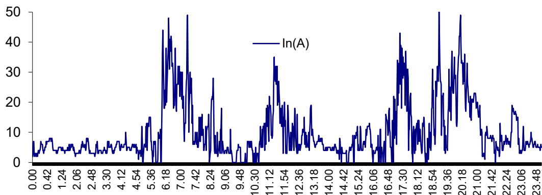
Figure 15. The behaviour of currents in the neutral.
