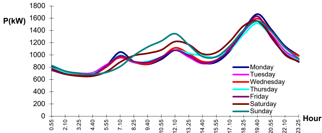
Figure 10. Average demand graph for days of the week.
