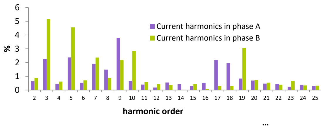
Figure 18. The behaviour of the levels according to the order of the current harmonic.
